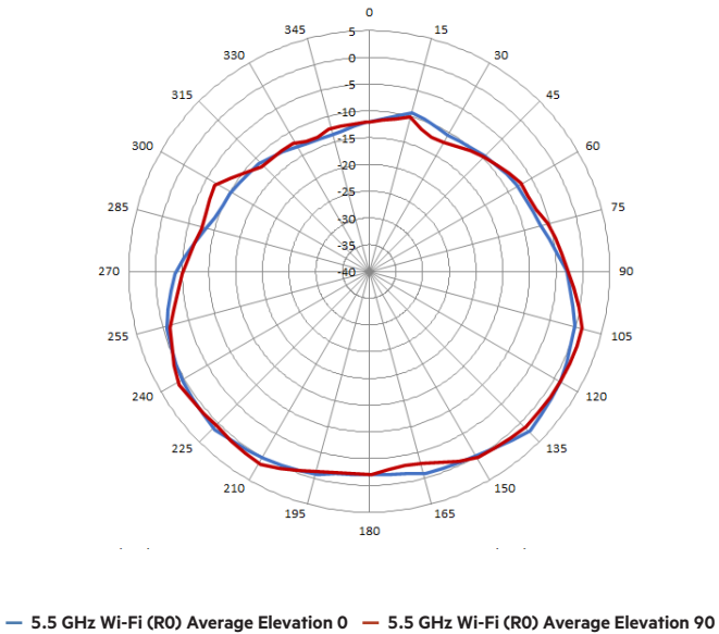
Figure 5. 5.5 GHz Wi-Fi antenna patterns (vertical)
