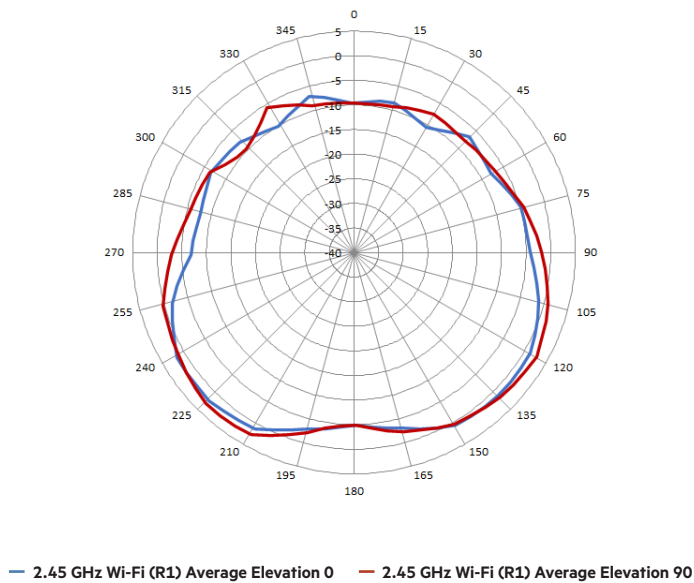
Figure 4. 2.45 GHz Wi-Fi antennas patterns (vertical)
