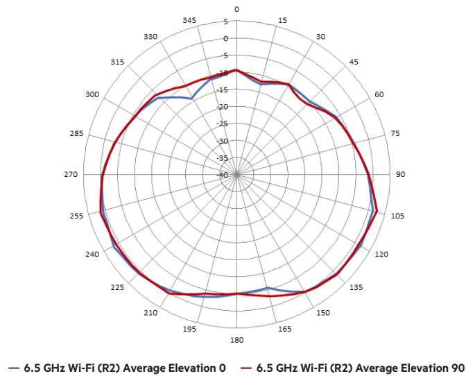
Figure 6. 6.5 GHz Wi-Fi antennas patterns (vertical)
